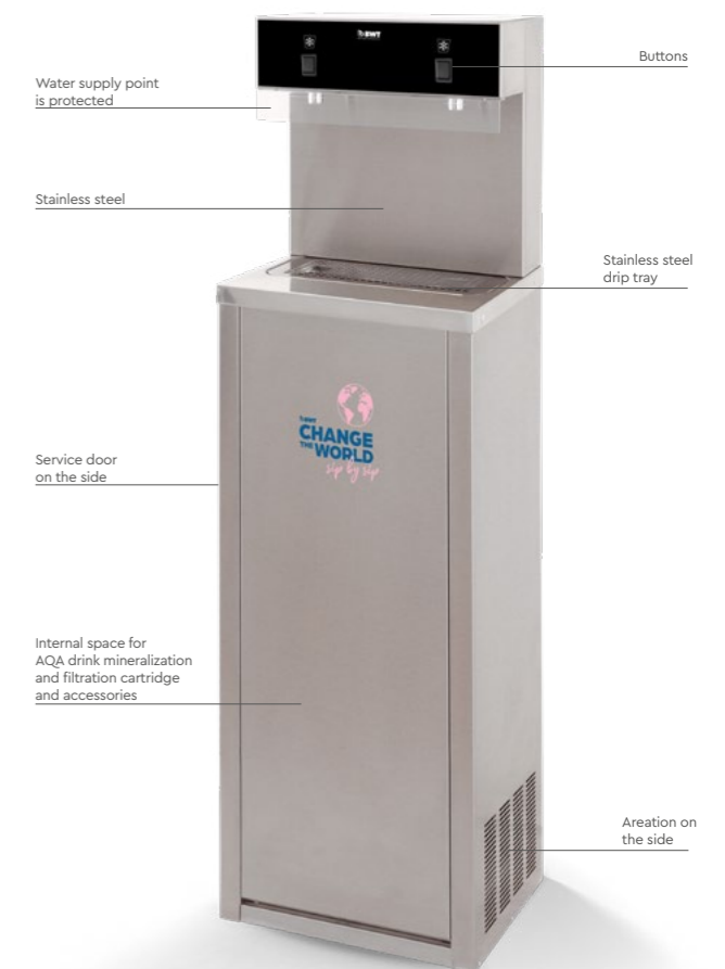
Hygienic and safe dispensing area
