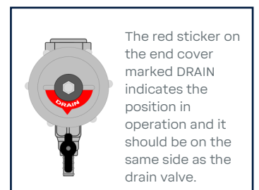
Right Side Installation
